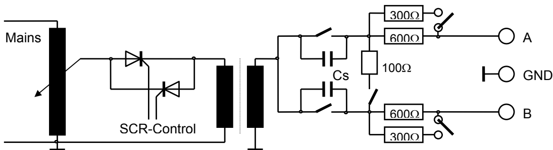
Fig. 1: POWER INDUCTION GENERATOR PIG 1500, schematic
